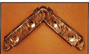
TDF Corners to suit TDF Roll-Formed Duct 25mm x 16ga - Galvanised Steel Product Code # 1243/1 Carton Quantity 500
