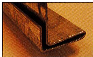
Reinforced Drive Cleat-RDC 3 metre length, 20ga Roll-Formed Galvanised Steel Product Code # 1222
