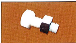
Fire Damper Low Melting Point Nylon Bolts. Melting Point Temperature Below 500 Deg. C. For Use with TDF / TDC Flange Channel Connections Product Code # 4908/1
