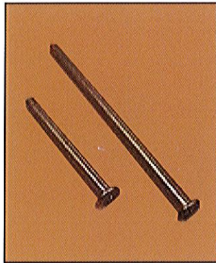
.105 KCD CD pin To suit CD1000 type weld guns Sizing from 0.5" to 4.25"
