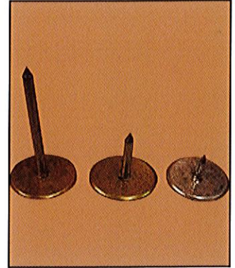
Duro-dyne weld rib pin Sizing from 0.5" to 4" Gold Seal prevents arcing
