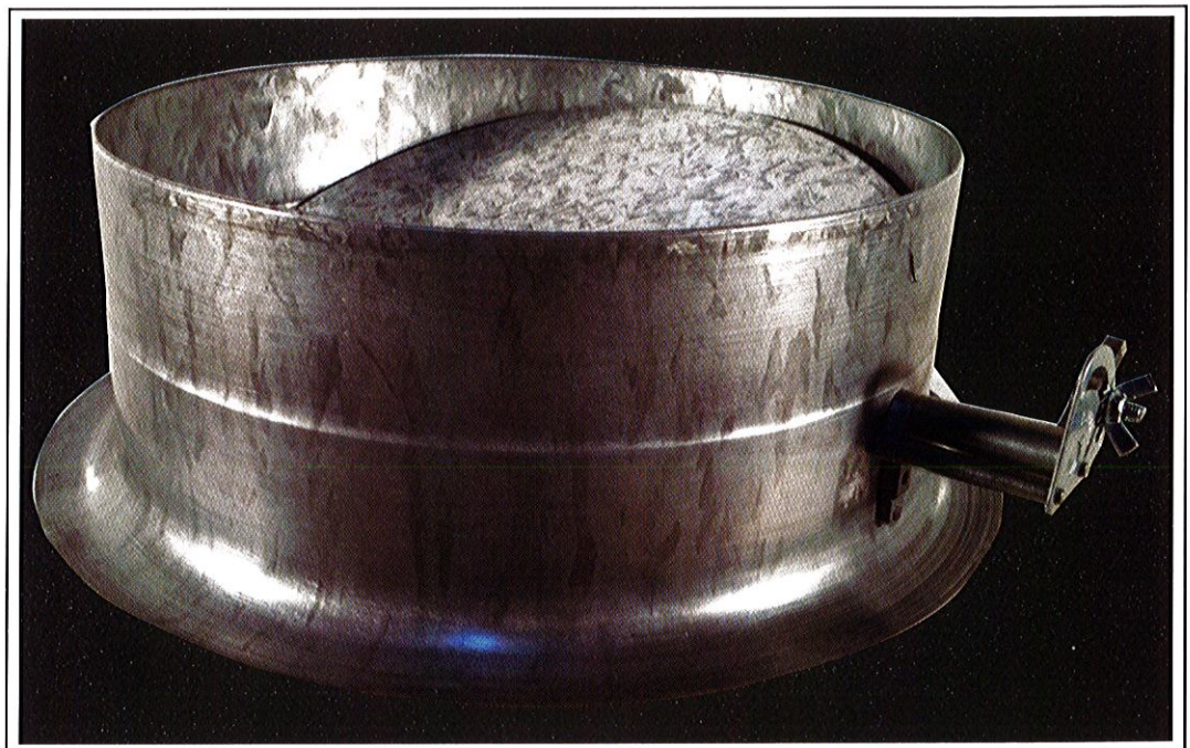
Model GSS1 - Flanged barrel complete with raised die cast quadrant, bearings and galvanised blade.
